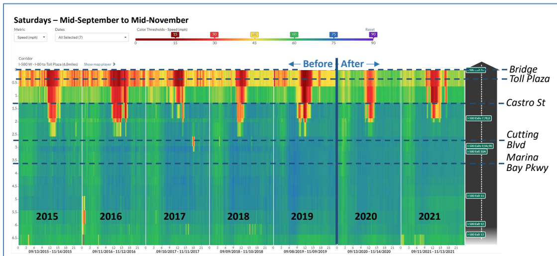
Figure 8-52: Speed Maps – I-580 West – Richmond Approach – Saturdays, Fall 2015-2021
