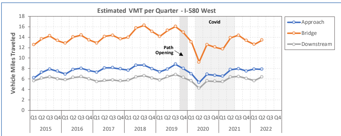
Figure 10-3: Estimated Vehicle Miles of Travel for Analysis Sections – I-580 West
