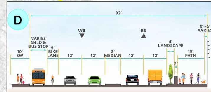
ON GRADE CONDITION
